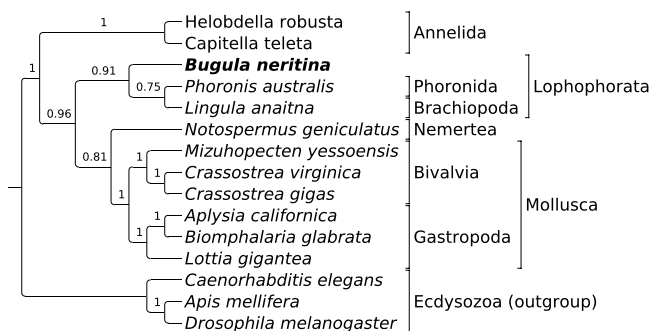
Fig. 2 Coalescent species tree of Lophotrochozoa (Spiralia) inferred from 57 BUSCO ML phylogenies. Branch supports measured as local posterior probabilities.
