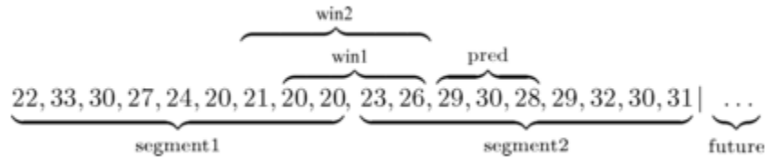
Figure 12. DyFor GP sliding window example, 3 of 5.
