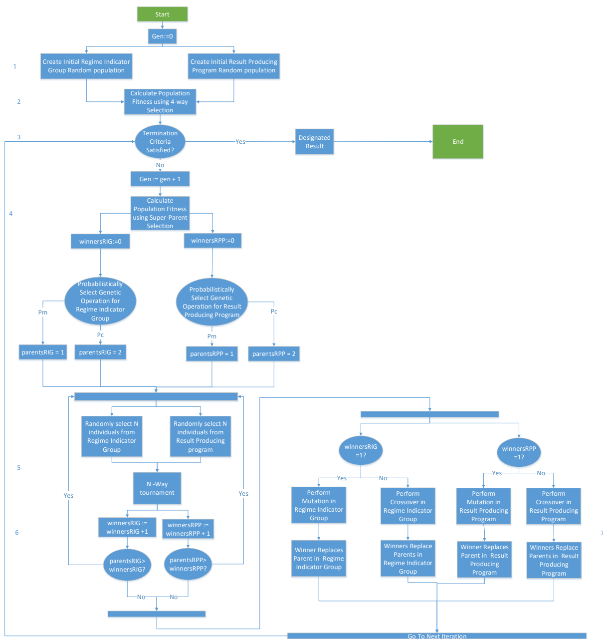
Figure 21. ADT algorithm flow chart.
