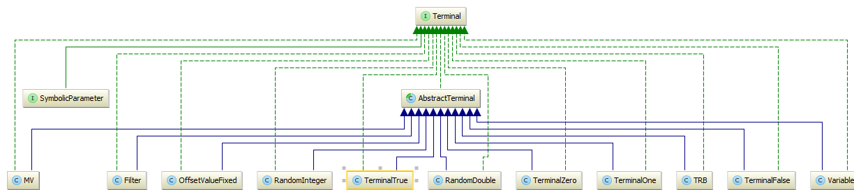
Figure C2. Primitive terminals class diagram.
