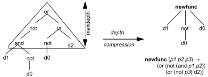
Figure 26. Module acquisition compression operation. A depth limited subtree is extracted and a new function, newfunc, is defined. newfunc includes parameters for each branch not included in the function because of the depth limit. Taken from (Angeline, 1994, p. 13).
