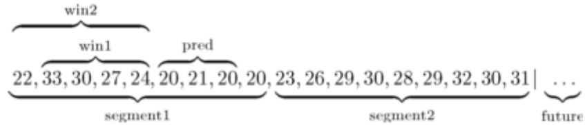
Figure 11. DyFor GP sliding window example, 2 of 5.
