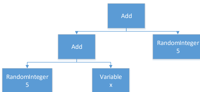
Figure 33. Java implementation of a sample S-expression tree.
