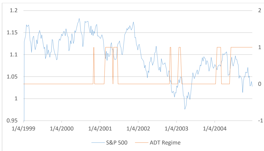
Figure H20. Regime predicted by best performing ADT individual for 1999-2004 period with transaction costs, plotted against normalized series.
