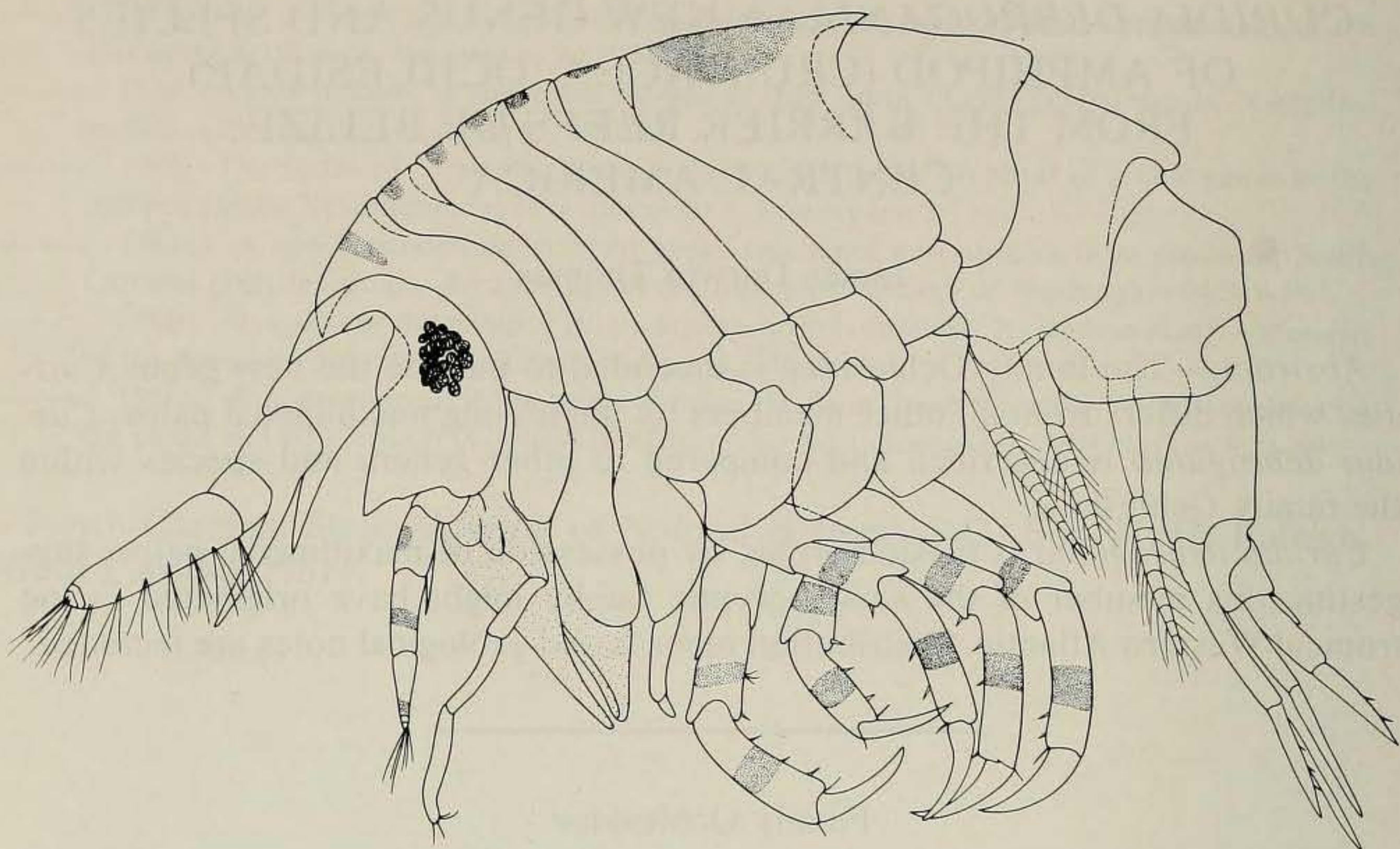
Fig. 1. Curidia debrogania , holotype, male, 1.59 mm, JDT Bel 48, Carrie Bow Cay, Belize.
