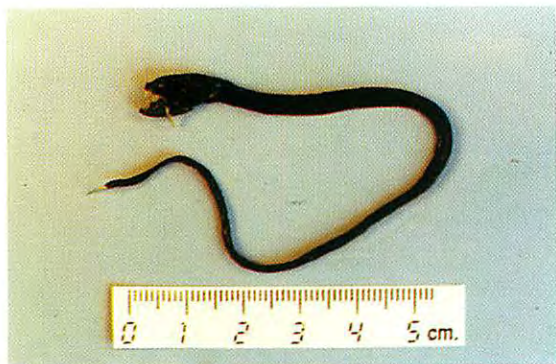
Idiacanthus fasciola
